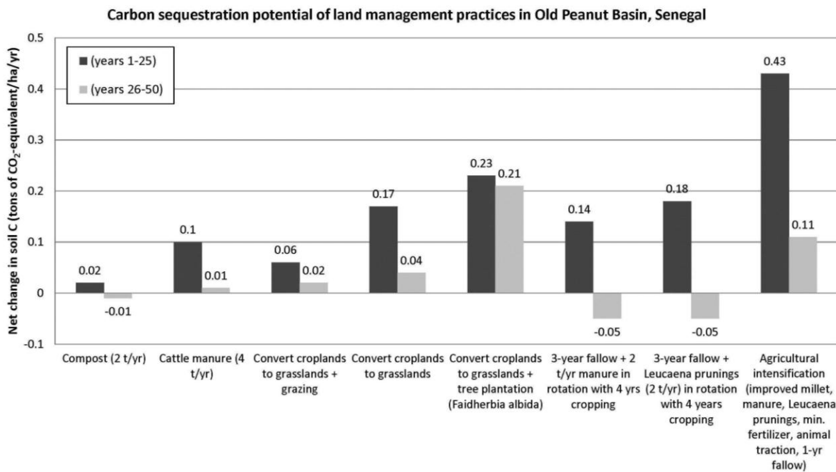
Figure 5. Soil carbon sequestration potential (in tons of CO 2 -eq/ha/yr) of different combinations of agricultural practices that may be used in CA. The graph reports results from the CENTURY model of agricultural yield, soil, and carbon dynamics, run for the Old Peanut Basin of Senegal, a semi-arid region (350-700 mm of annual rainfall) in which major crops include millet, groundnuts, sorghum, and cowpea. Figure is drawn from data presented in FAO, 2004.
